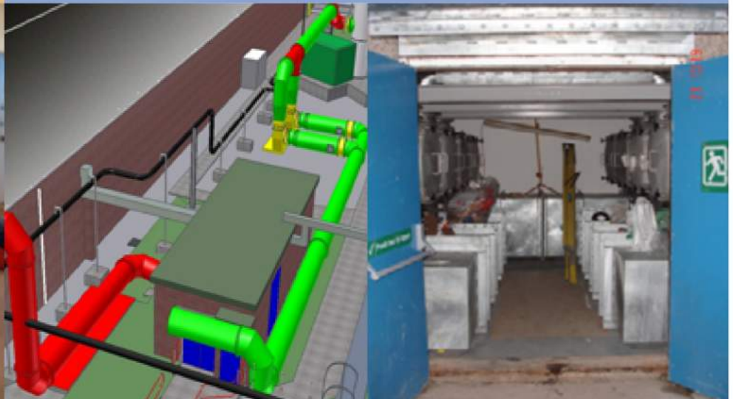
New Ventilation Discharge Route with HEPA filters for Dounreay
